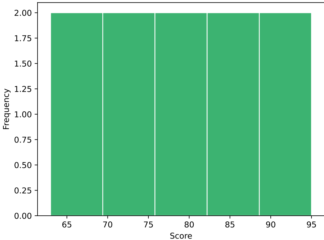
Score Distribution
