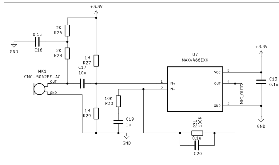
MICROPHONE AND AMPLIFIER
