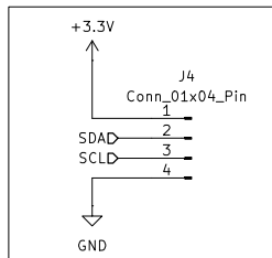
OLED display connector (I2C)
