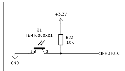
PHOTO SENSOR
