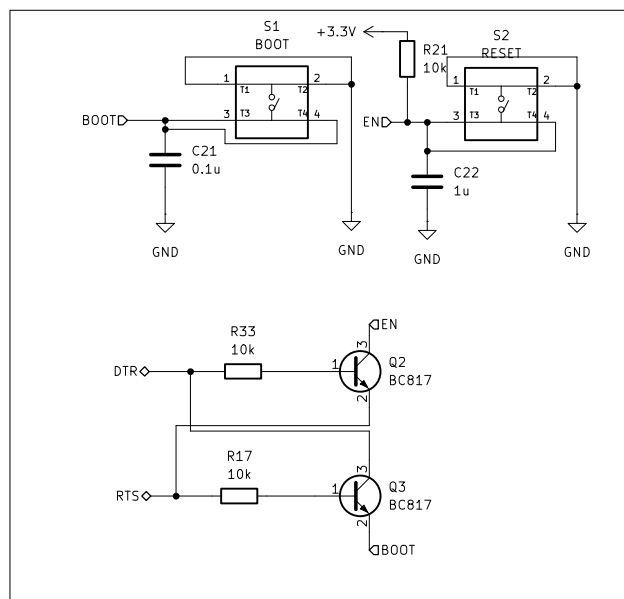
RESET and BOOT buttons
