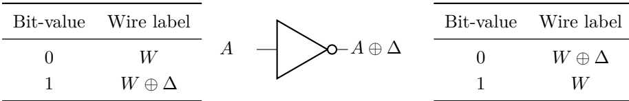
Figure 3.1: Wire label mappings before (left) and after (right) a NOT gate.
