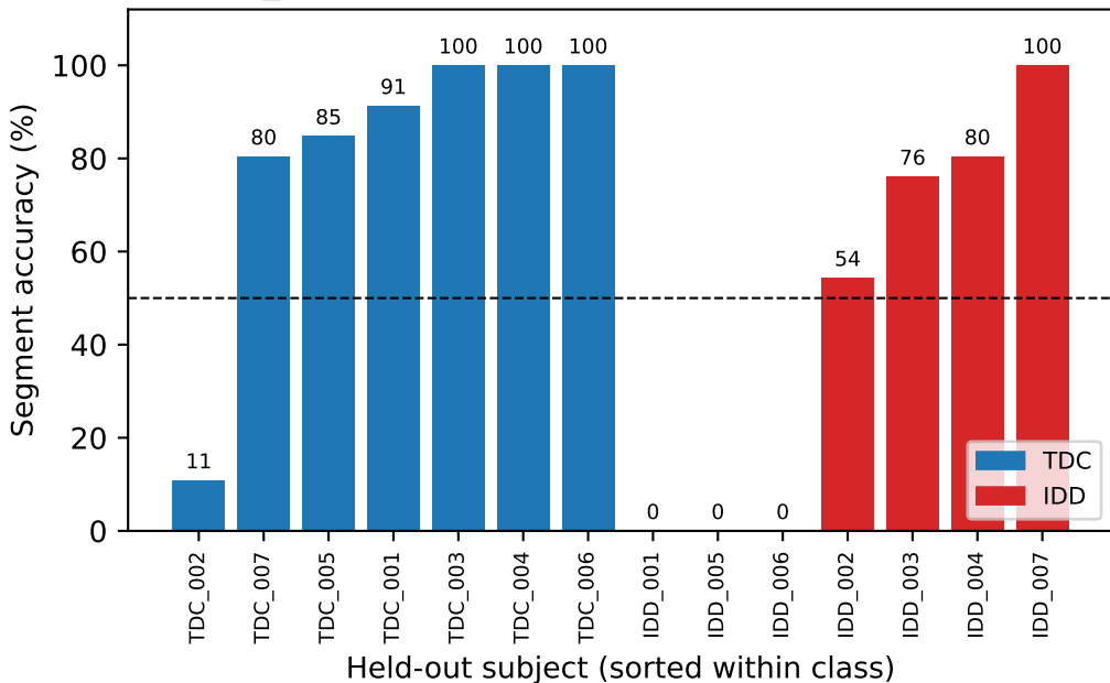
DS1_Rest: per-subject accuracy, subject-wise CV
