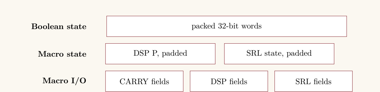
Figure 2: Separate Boolean and word-level memory areas.
