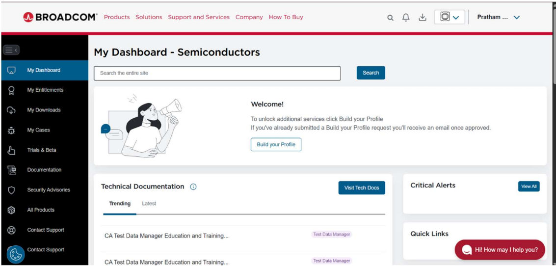
Fig 3.2: Broadcam dashboard
