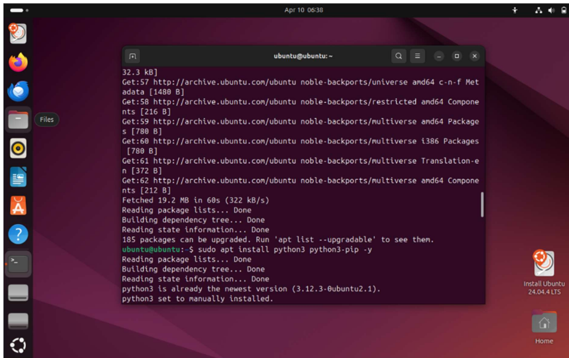
Fig 3.9: Installing Python
