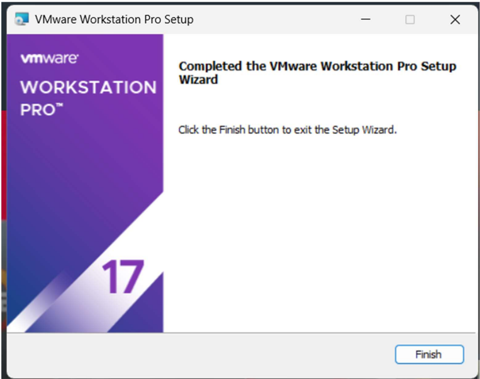
Fig 3.1: Workstation downloaded
