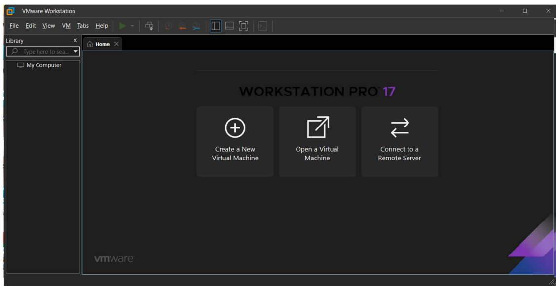
Fig 3.4: VMWare Dashboard
