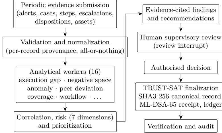
Figure 1: SAT-SA supervisory workflow as implemented. Analytics are deterministic; orchestration (direct worker or LangGraph) sequences the stages and pauses for the human decision.
