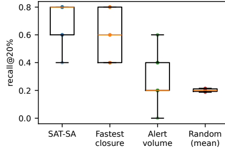
Fig. 2. Recall@20% of generator-labelled pathological entities across 20 generated populations (PR01). The generator injects behaviours that SAT-SA targets, so this is a controlled mechanism test, not an unbiased benchmark.
