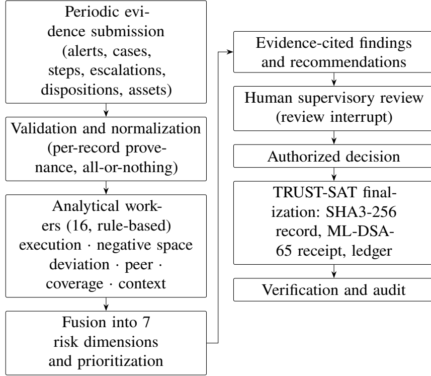
Fig. 1. SAT-SA supervisory workflow along the evaluated path. The analytical-worker stage is the evaluated subset of the registered agents (Table 2). All analytics are deterministic and rule-based; orchestration (direct worker or LangGraph) sequences the stages and pauses for the human decision.
