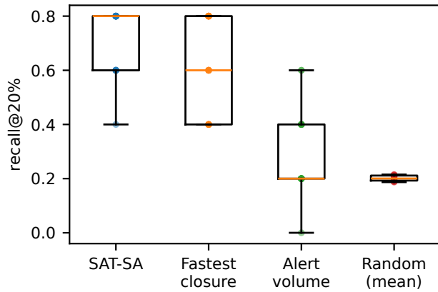
FIGURE 2. Recall@20% of generator-labelled pathological entities across generated populations (PR01).
