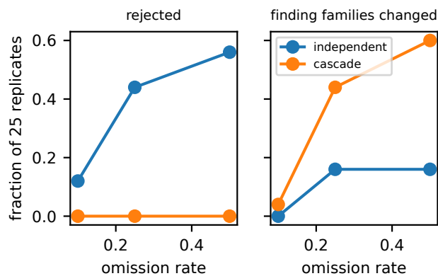
FIGURE 4. Record omission: independent omission is often rejected by all-or-nothing validation; referentially consistent omission is accepted and changes findings more often as the rate grows (R01b).
