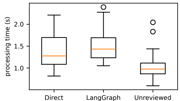
FIGURE 6. Workflow processing time by execution mode on one machine with SQLite (O01).
