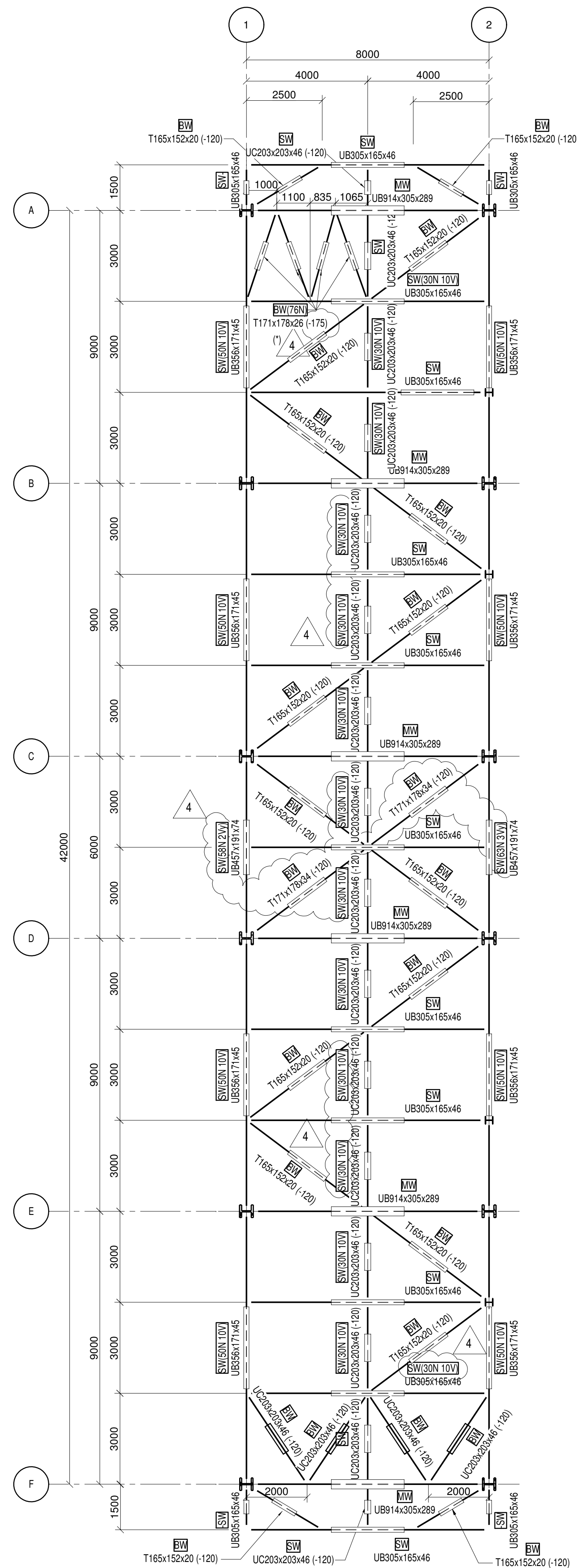
PLAN EL. 111.500 (T.O.S.) SCALE 1:100
