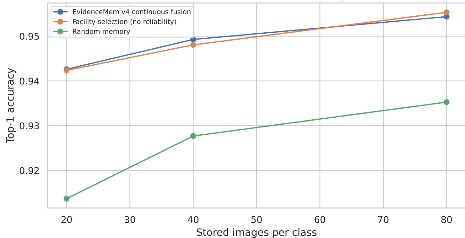
Matched memory budget: siglip2_b16_384
