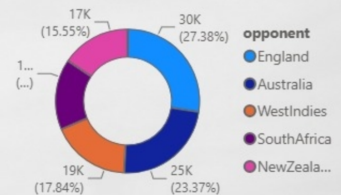
Total_Matches - Opponent
