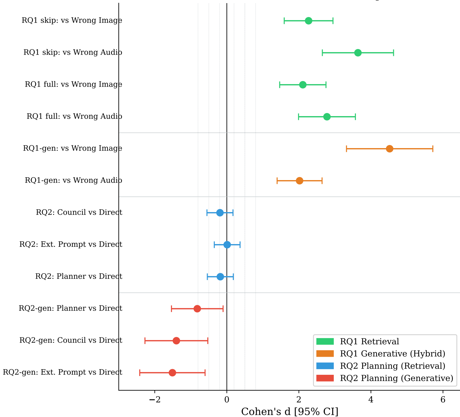
Forest Plot: Effect Sizes Across All Comparisons
