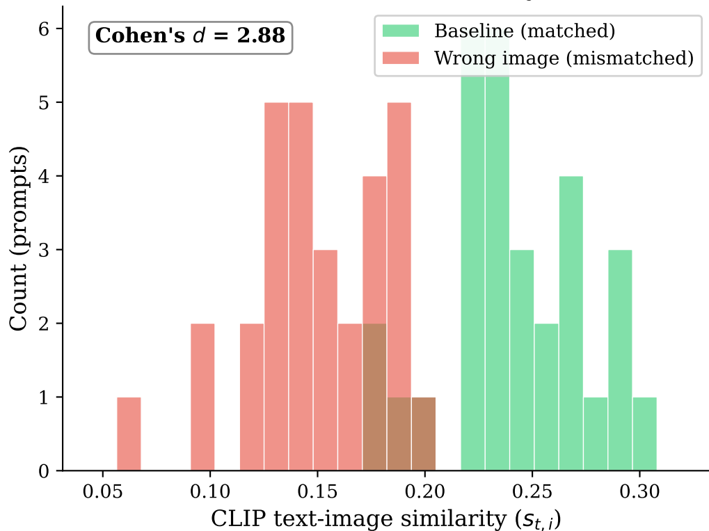
CLIP Channel Sensitivity
