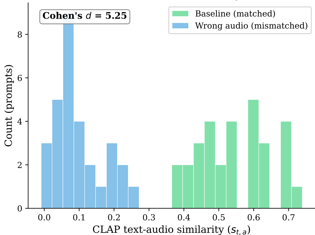
CLAP Channel Sensitivity
