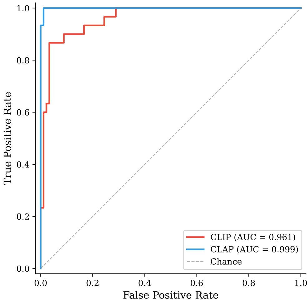
ROC: Matched vs Mismatched Discrimination
