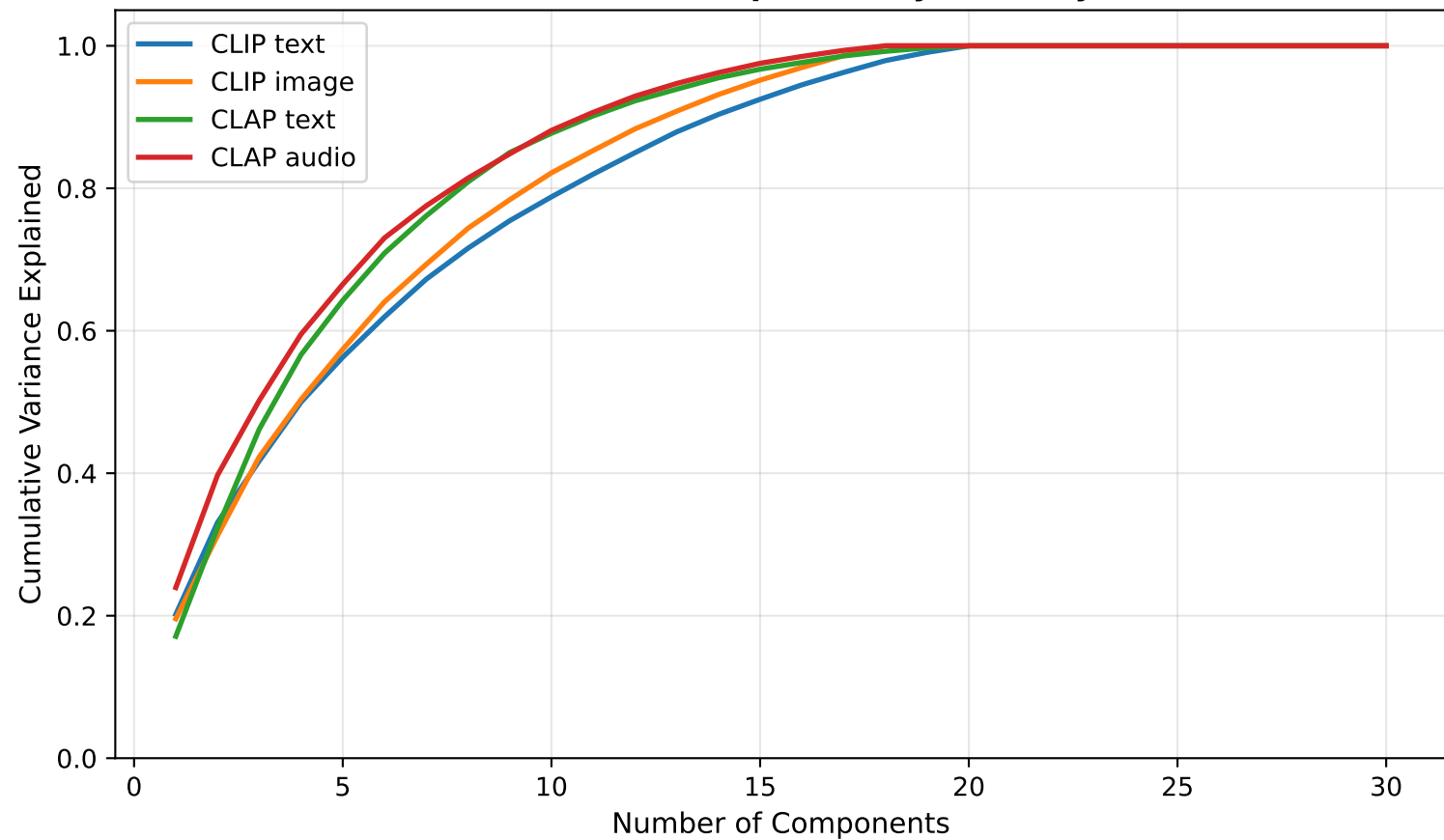
PCA Variance Explained by Modality
