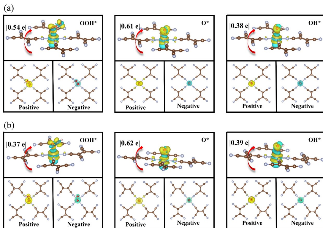
Figure S4 the differential charge density diagram of intermediates adsorbed on (a) Ru-pTCNE, and (b) Os-cTCNE substrate.
