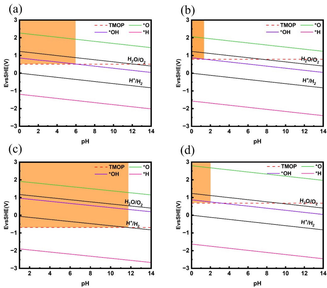
Figure S1 Surface Pourbaix diagrams for the electrochemical stability of (a) Ru-pTCNE, (b) Os-pTCNE, (c) Mn-cTCNE and (d) Os-cTCNE.
