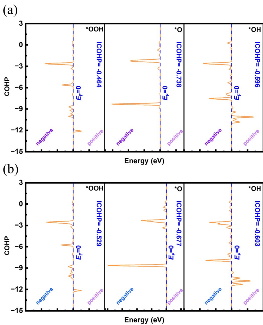
Figure S3 the COHP between the TM and O atoms : (a) Ru-pTCNE, and (b) Os-cTCNE.
