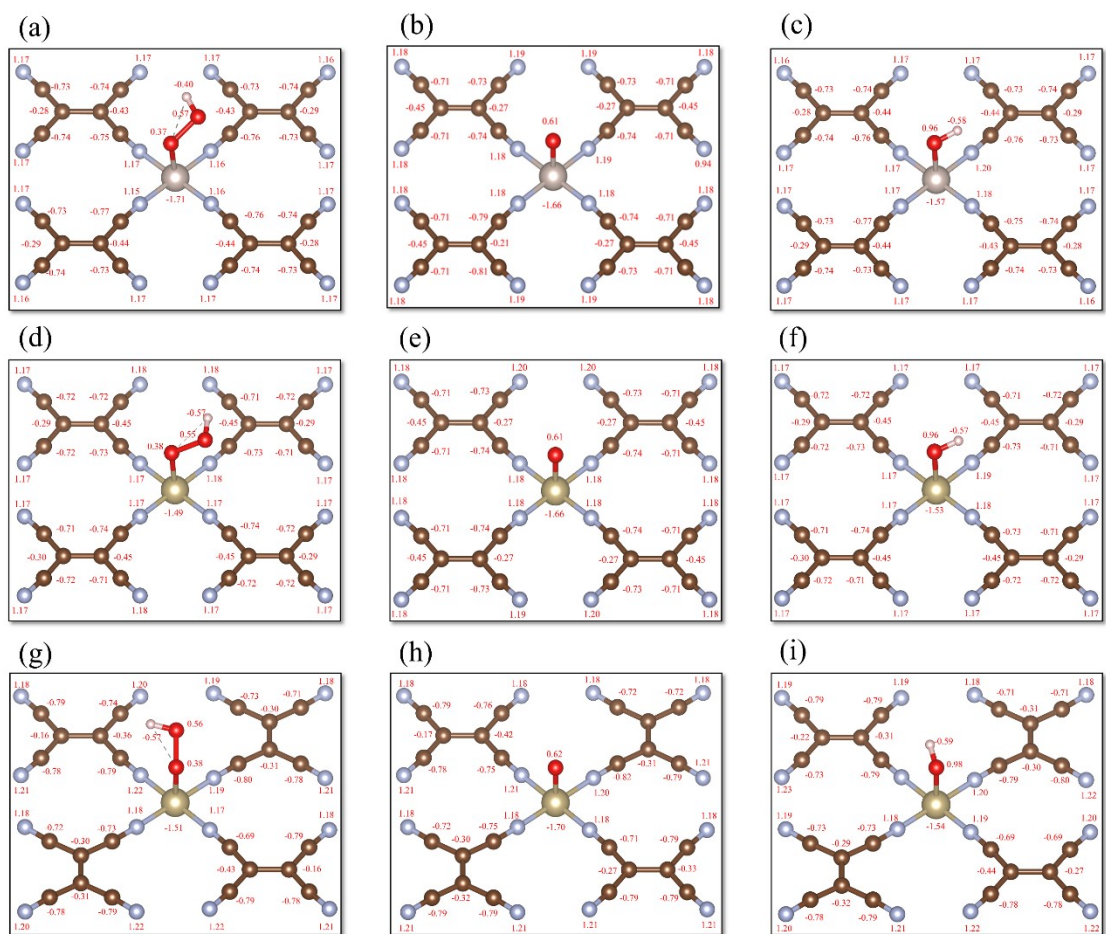
Figure S5 the Bader charge diagram of intermediates adsorbed on (a-c) Ru-pTCNE, (d-f) Os-pTCNE, and (g-i) Os-cTCNE substrate.
