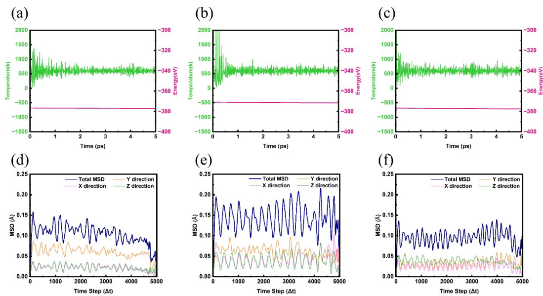
Figure S2 the AIMD and mean-square deviation (MSD) for the (a, d) Os-pTCNE, (b, e) Ru-pTCNE, and (c, f) Os-cTCNE.
