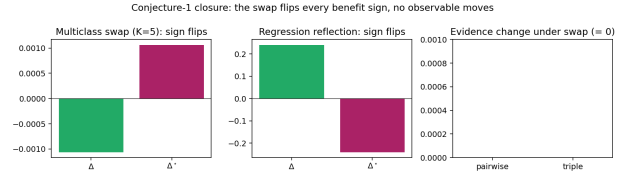
Fig. 14. Closing Conjecture 1 (Thm 4(iii)): the swap flips every benefit sign while no label-free observable of any order moves (exact zero).
