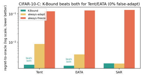
Fig. 15. CIFAR-10-C frontier (regret-to-oracle, log scale). KGA (teal) is strictly below both always-adapt and always-freeze for Tent and EATA (“beats both”) at a 0% false-adapt rate, and ties always-adapt for the robust SAR candidate. Bars are the exact values of Table XVIII, rendered by scripts/make_appendix_frontier_figs.py from results/decisive_tta_results.json.
