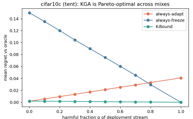
Fig. 9. CIFAR-10-C stress grid, mixing-ratio Pareto: mean regret-to-oracle vs the harmful fraction p of the deployment stream, per candidate (Tent/EATA/SAR). KGA (green) stays on the Pareto front—tying always-adapt at p=0 , strictly beating both trivial policies for p \gtrsim p^* , and never collapsing like always-adapt or stalling like always-freeze.
