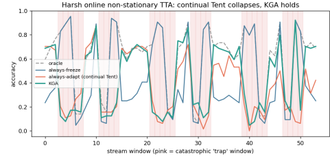
Fig. 7. Per-window accuracy on the harm-dominated stream (pink = catastrophic “trap” windows). Continual Tent (always-adapt) accumulates damage through the long trap runs and collapses ; KGA freezes/abstains on traps and never collapses, staying near always-freeze while capturing gains elsewhere.
