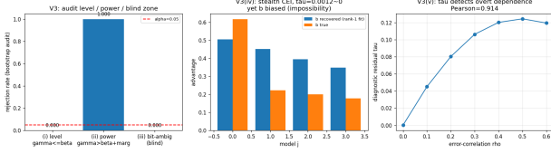
Fig. 12. The budget audit (Thm 4(iv)): sound at level \alpha , power 1.000 beyond the radius, correctly blind exactly on the bit-ambiguous set and the rank-one-preserving stealth law.
