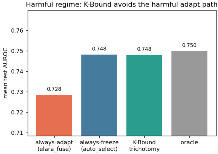
Figure 7.1: KGA in the harmful-fusion regime. The certificate almost entirely blocks the legacy-fuse candidate; regret-to-oracle falls from 0.0214 (always-adapt) to 0.0019 ( \approx 11\times reduction). Source: kbound_harmful_results.json .
