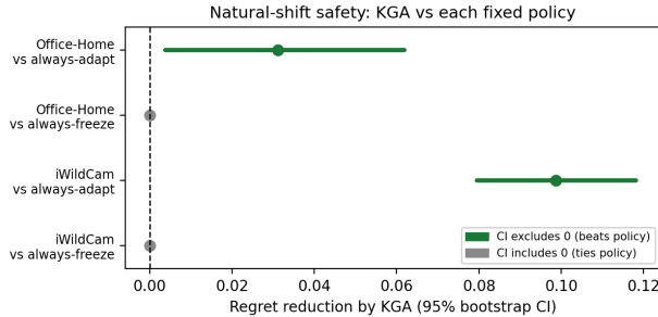
Figure 7: Natural-shift no-harm, not beats-both. Positive values favor KGA. Office-Home and iWildCam beat always-adapt but tie always-freeze under the corrected out-of-fold replay; the intervals are paired held-out-condition bootstrap intervals from the saved OOF bootstrap lock (App. I).
