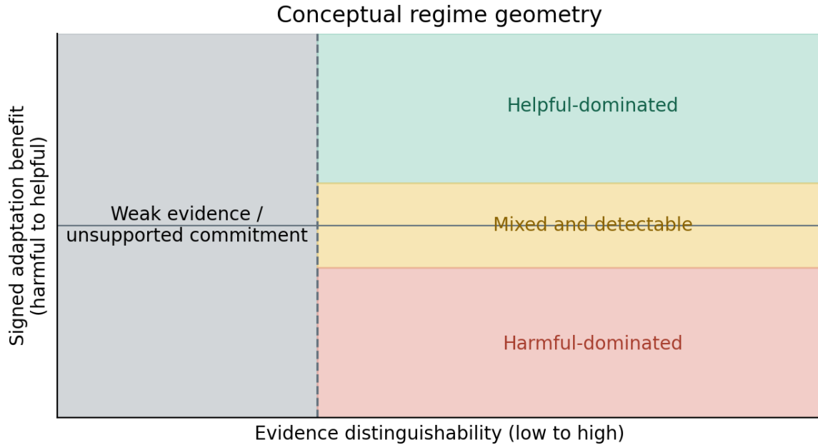
Figure 4: Regime geometry for K-Bound. The important axis is not dataset name but where the deployment sits relative to the frontier. Helpful- or harmful-dominated regimes usually produce no-harm ties with the better fixed policy; low-margin regimes force abstention; mixed and detectable regimes are where a valid adapt/freeze/abstain router can beat both fixed policies. This is a conceptual schematic : axis positions are illustrative regime categories, not measured coordinates (the actual per-track verdicts are in Table 1).
