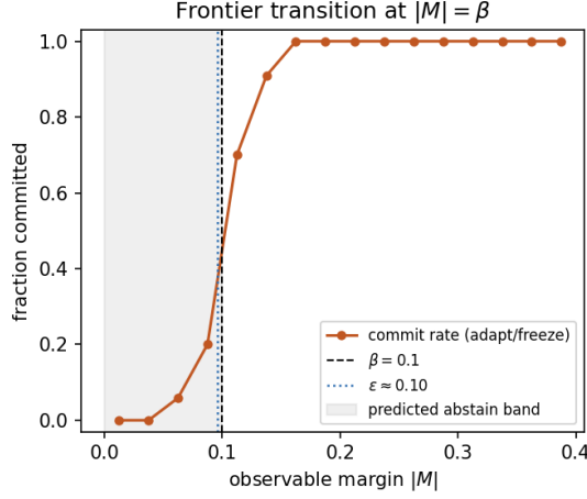
Figure 5: Measured benefit-sign frontier (synthetic ground truth, archived cross-fitted rule). The commit rate transitions sharply from abstention to adapt/freeze near |M|=\beta ; the calibrated radius \varepsilon (dotted) approximately tracks \beta in this construction. Companion panels—estimator recovery and \text{FA}_u \leq \alpha across \beta —in fig_frontier_recovery.png , fig_frontier_fa_coverage.png .
