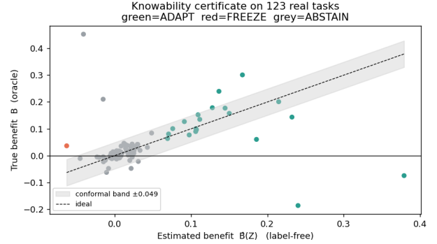
Figure 3: The certificate rule in one picture. KGA estimates the label-free benefit \hat{\Delta}(Z) and forms an interval \hat{\Delta} \pm \varepsilon : if the interval is entirely positive it adapts, if entirely negative it freezes, and otherwise it abstains. The vertical axis here uses true benefit only for offline audit; deployment decisions use only unlabeled evidence and the pre-calibrated radius.
