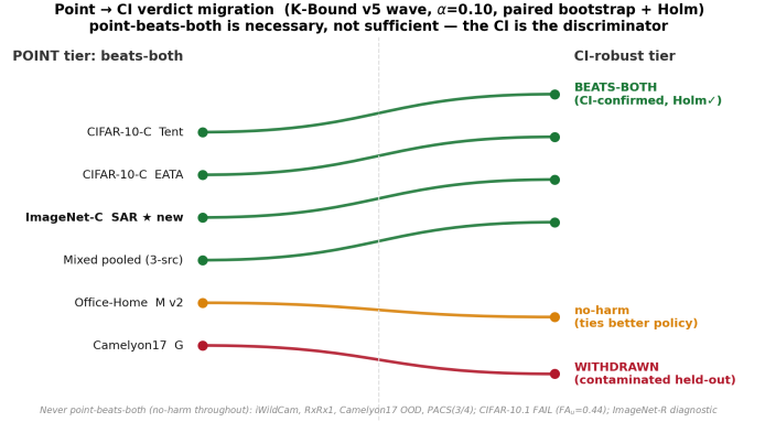
Fig. 8. Point → CI verdict migration for the confirmatory wave ( \alpha=0.10 ; paired per-condition bootstrap, Holm-corrected across the wave). Point-beats-both is necessary but not sufficient: under the CI, only CIFAR-10-C Tent/EATA, the constructed three-source mixture, and ImageNet-C SAR remain beats-both; Office-Home’s point edge migrates to no-harm, and the contaminated Camelyon17 Protocol-G arm stays withdrawn. ImageNet-C SAR is the arm newly CI-confirmed in this fold-in pass. Reproducibility : verdicts from scripts/uniform_scorer.py + scripts/percondition_bootstrap.py ( B=5000 ), scored once against the frozen bars in results_source.json .
