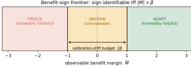
Fig. 2. The benefit-sign frontier. The sign of the adaptation benefit is identifiable from label-free evidence iff the population margin |M| exceeds the calibration-drift budget \beta . Outside the band KGA ADAPTS (knowably helpful) or FREEZES (knowably harmful); inside the band (the unknowable region), abstention is information-theoretically forced. (This is the population identifiability frontier of Theorem 2; the deployed finite-sample rule instead thresholds \hat{\Delta} \pm \varepsilon , Fig. 3.)
