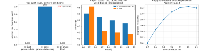
Fig. 10. Budget audit (Synthetic validator; Thm. 5(iv)).
