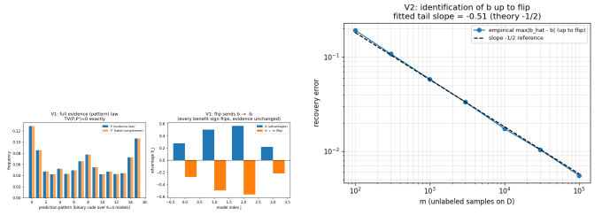
Fig. 9. One-bit identification (Synthetic validator; Thm. 5(ii)).
