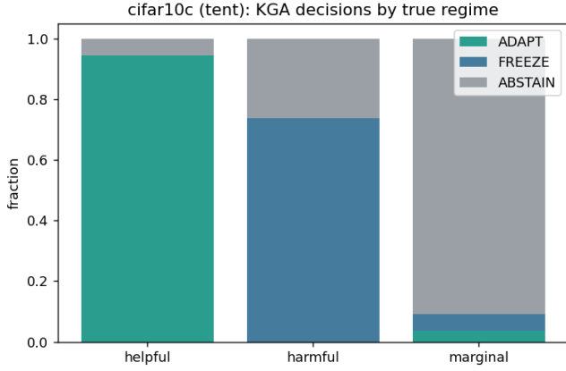
(a) decisions by true regime
