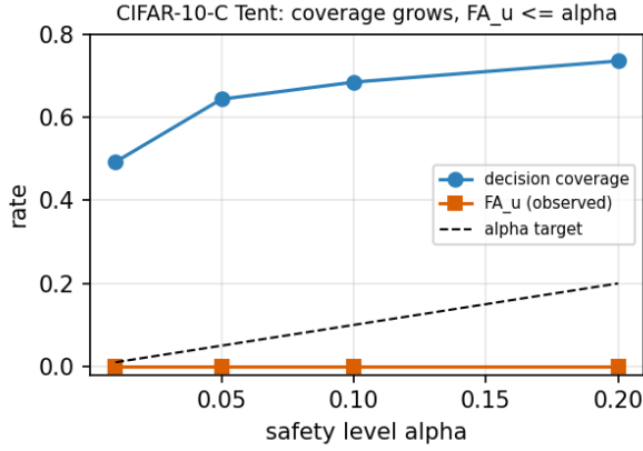
Fig. 7. The safety knob. Sweeping the level \alpha trades decision coverage against the false-adapt rate: the certificate holds false-adapt at or below target while coverage grows with \alpha , so a deployer chooses the operating point rather than accepting a fixed one.
