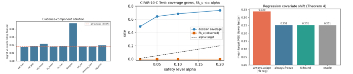
Fig. 5. Left: evidence-component ablation (disagreement dominates). Middle: \alpha sweep—safety vs coverage. Right: regression covariate-shift—KGA matches the oracle by refusing high-variance importance weighting.
