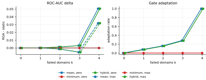
Fig. 13. T3 validation: RGA adaptation rate and ROC-AUC delta as a function of the number of corrupted domains k .
