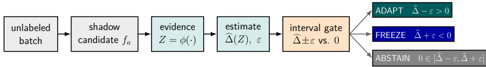
Figure 1: KGA’s empirical decision flow for one evaluation cell. A shadow adapter creates f_a from frozen f_0 . Labeled development cells fit the benefit predictor, and disjoint residual-calibration cells determine its error radius. The scored cell contributes label-free evidence only. An interval above zero selects ADAPT, one below zero selects FREEZE, and an interval crossing zero selects ABSTAIN. The figure defines the action rule; it does not establish interval coverage.
