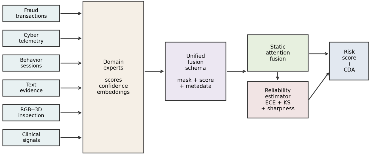
Fig. 1. ELARA system architecture. Domain experts produce scores, confidence values, and compact embeddings; a unified fusion schema feeds static attention and the RGA reliability estimator; the system emits a risk score and counterfactual domain attribution.
