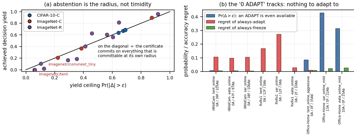
Fig. 5. Abstention is the radius, not timidity. (a) Achieved decision yield against the ceiling \mathbb{P}(|\Delta| > \varepsilon) ; points on the diagonal commit on everything committable at their own radius. (b) On the natural tracks the critique names, the fraction of cells on which an ADAPT is even available at the published radius, against the regret of the two fixed policies. On RxRx1 and iWildCam that fraction is \leq 0.007 , and the certificate’s value is carried entirely by its FREEZE commitments.
