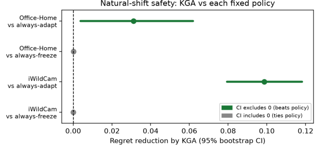
Fig. 7. Natural-shift action safety. Positive values favor KGA. Office-Home and iWildCam beat always-adapt but tie always-freeze under the corrected out-of-fold replay; the intervals are paired held-out-condition bootstrap intervals from the saved OOF bootstrap lock (App. J).
