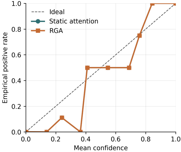
Fig. 12. Reliability diagram for static attention and RGA.
