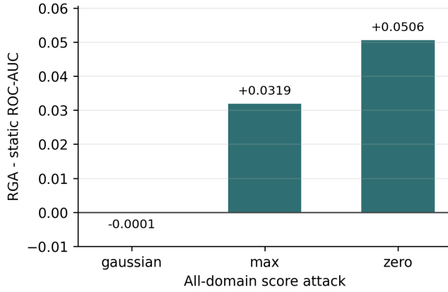
Fig. 11. All-domain adversarial ROC-AUC delta between RGA and static attention. Complete single-domain scenarios are reported in Table XX.
