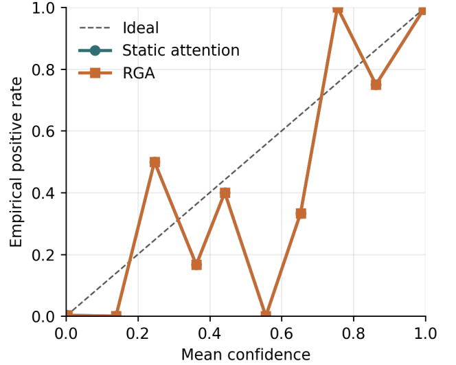
Fig. 13. Reliability diagram for static attention and RGA.
