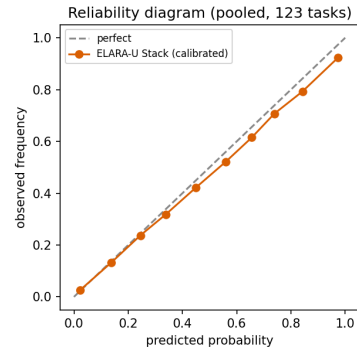
Fig. 1. Reliability diagram for the isotonic-calibrated ELARA Stack, pooled over 123 tasks (calibrator fit on validation only). Points near the diagonal indicate good calibration; Brier/NLL in Table X.
