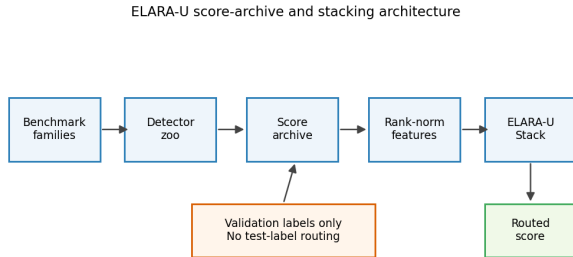
Fig. 3. ELARA architecture: benchmark families feed a detector zoo and score archive; validation-only labels and unlabeled deployment scores drive the router.
