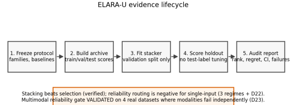
Fig. 5. Router decision lifecycle and evidence boundary. Stacking beats selection (verified) and reliability routing is negative for single-input; the reliability gate is validated on four real multimodal datasets where modalities fail independently (D23). Sealed external evidence still bounds any universal-SOTA claim.
