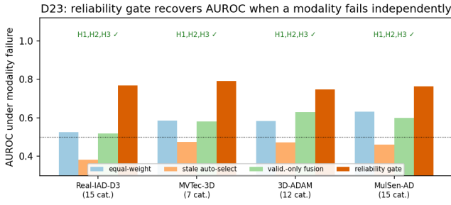
Fig. 2. Multimodal independent-modality-failure regime (D23) on four real datasets under the canonical noise protocol. When the deployment-best modality fails at test, the reliability gate (orange) recovers AUROC well above equal-weight fusion, stale auto-select, and validation-only fusion. “H1,H2,H3 ✓” marks datasets where all three pre-registered hypotheses pass — all four do. Authoritative deltas and CIs in Table XIX.
