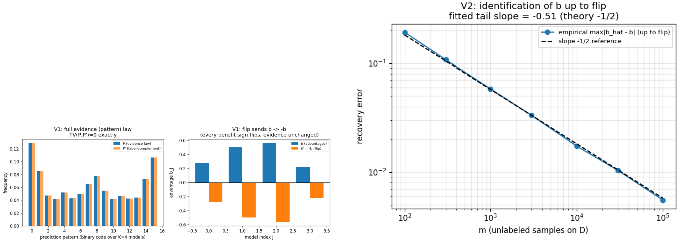
Fig. 10. One-bit identification (Synthetic validator; Thm 4(ii)): the label complement matches the full evidence law (TV = 0) while negating every advantage (left); recovery of b up to the bit at the m^{-1/2} rate (right).
