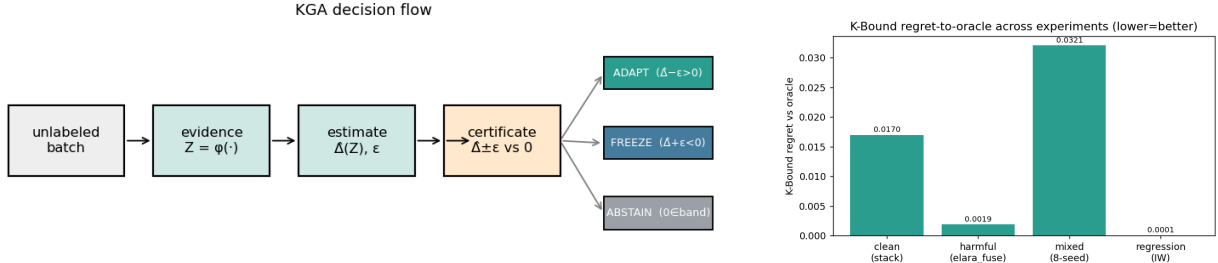
Figure 8: Left: the KGA decision flow (evidence \rightarrow estimate \rightarrow certificate \rightarrow adapt/freeze/abstain). Right: KGA regret-to-oracle across all experiments.
