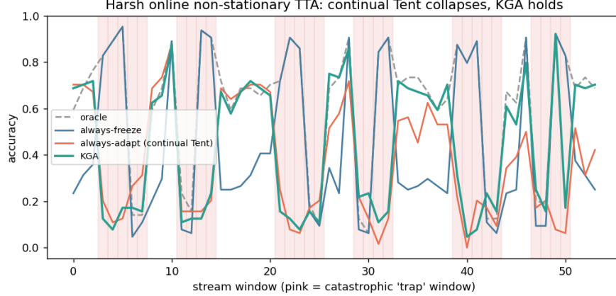
Figure 9: Per-window accuracy on the harm-dominated stream (pink = catastrophic “trap” windows). Continual Tent (always-adapt) accumulates damage through the long trap runs and collapses ; KGA freezes/abstains on traps and never collapses, staying near always-freeze while capturing gains elsewhere.
