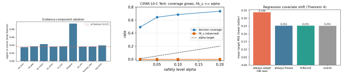
Fig. 5. Left: evidence-component ablation (disagreement dominates). Middle: \alpha sweep—safety vs coverage. Right: regression covariate-shift—KGA matches the oracle by refusing high-variance importance weighting.
