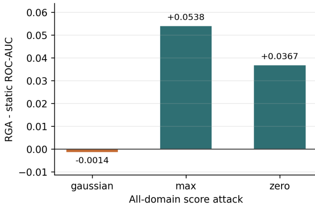
Fig. 11. All-domain adversarial ROC-AUC delta between RGA and static attention. Complete single-domain scenarios are reported in Table XXII.
