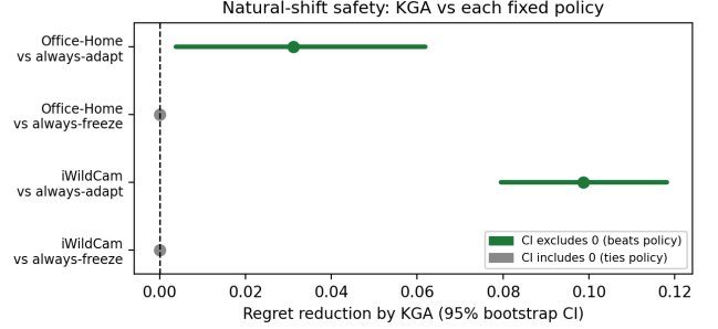
Fig. 7. Natural-shift no-harm, not beats-both. Positive values favor KGA. Office-Home and iWildCam beat always-adapt but tie always-freeze under the corrected out-of-fold replay; the intervals are paired held-out-condition bootstrap intervals from the saved OOF bootstrap lock (App. I).
