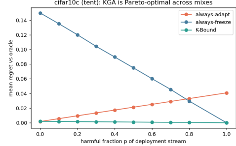
Fig. 3. CIFAR-10-C stress grid: regret-to-oracle vs harmful fraction p per candidate. KGA ties always-adapt at p=0 and beats both for p \gtrsim p^* .
