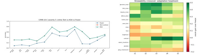
Fig. 8. CIFAR-10-C. Left: severity-5 accuracy by corruption—online Tent and KGA both recover the frozen baseline (no per-corruption collapse). Right: knowability crossover map—adaptation headroom (oracle gain over freeze) by corruption \times severity; large on noise/blur, small on easy corruptions (brightness), matching where \Delta is large.
