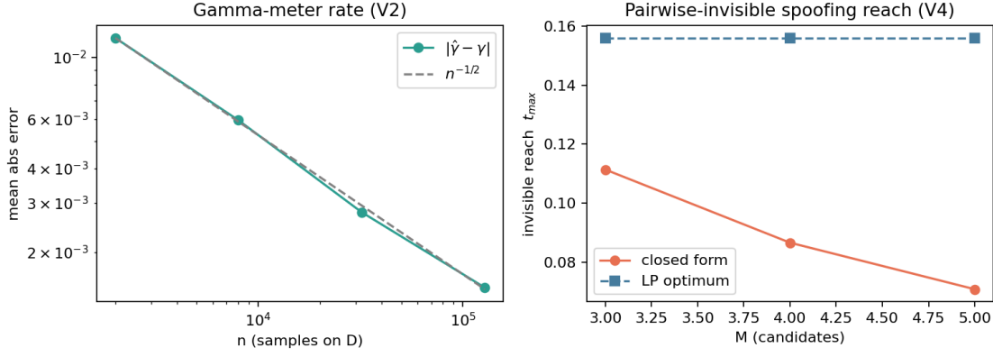
Figure C.5: The \gamma -meter and the agreement-invisible reach. Left: |\hat{\gamma} - \gamma| decays at the proven n^{-1/2} rate (Theorem C.4). Right: the constructive invisible reach t_{\max} (closed form) versus the exact LP reach over all pairwise-agreement-preserving couplings; the LP reach does not shrink with M — only richer (third-order) evidence shrinks it (Proposition C.16).
