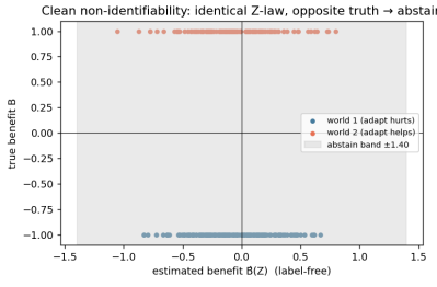
Fig. 2. Clean non-identifiability witness (Synthetic): identical Z -law (KS p > 0.05 on all features), exactly opposite true benefit, 100% abstention. Empirical realization of Theorem 1.
