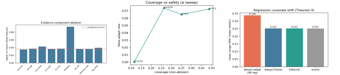
Fig. 5. Left: evidence-component ablation (disagreement dominates). Middle: \alpha sweep—safety vs coverage. Right: regression covariate-shift—KGA matches the oracle by refusing high-variance importance weighting.
