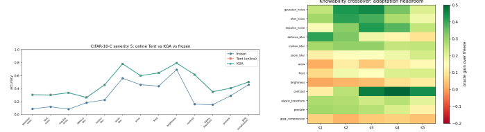
Fig. 7. CIFAR-10-C. Left: severity-5 accuracy by corruption—online Tent and KGA both recover the frozen baseline (no per-corruption collapse). Right: knowability crossover map—adaptation headroom (oracle gain over freeze) by corruption \times severity; large on noise/blur, small on easy corruptions (brightness), matching where \Delta is large.
