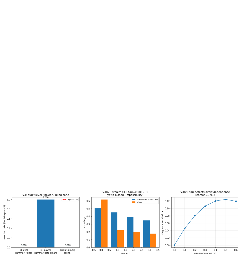
Fig. 11. The budget audit (Synthetic validator; Thm 4(iv)): sound at level \alpha , power 1.000 beyond the radius, correctly blind exactly on the bit-ambiguous set and the rank-one-preserving stealth law.
