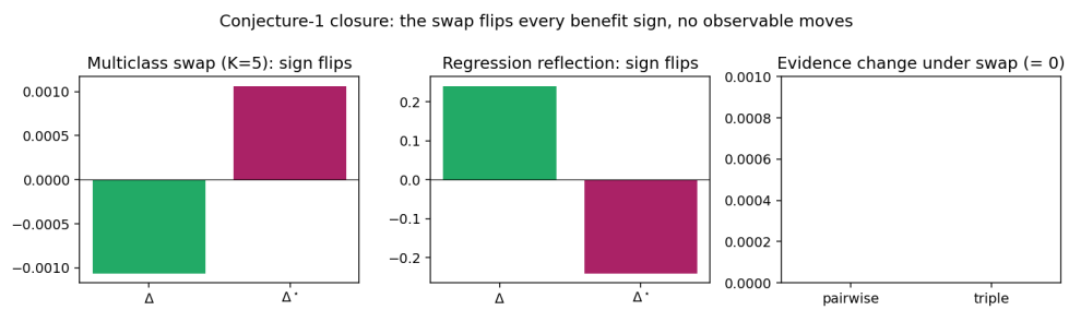
Fig. 13. Closing Conjecture 1 (Synthetic validator; Thm 4(iii)): the swap flips every benefit sign while no label-free observable of any order moves (exact zero).
