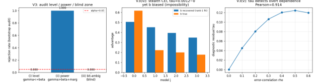
Fig. 4. Budget audit (Synthetic validator; Thm. 5(iv)).
