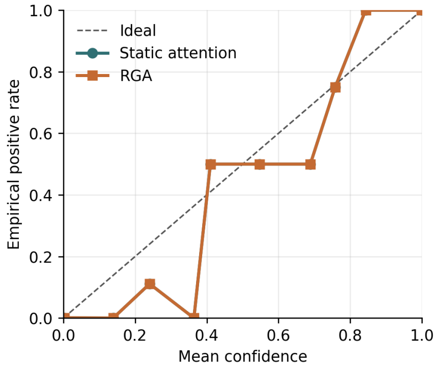
Figure 6: Reliability diagram for static attention and RGA.
