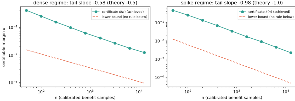
Figure 19: The knowability rate (Theorems 22–23). Achieved certifiable margin of the deployed empirical-Bernstein certificate versus the two-point lower bound, in the dense ( n^{-1/2} ) and spike ( n^{-1} ) regimes; slopes match and the offset is a bounded universal constant.
