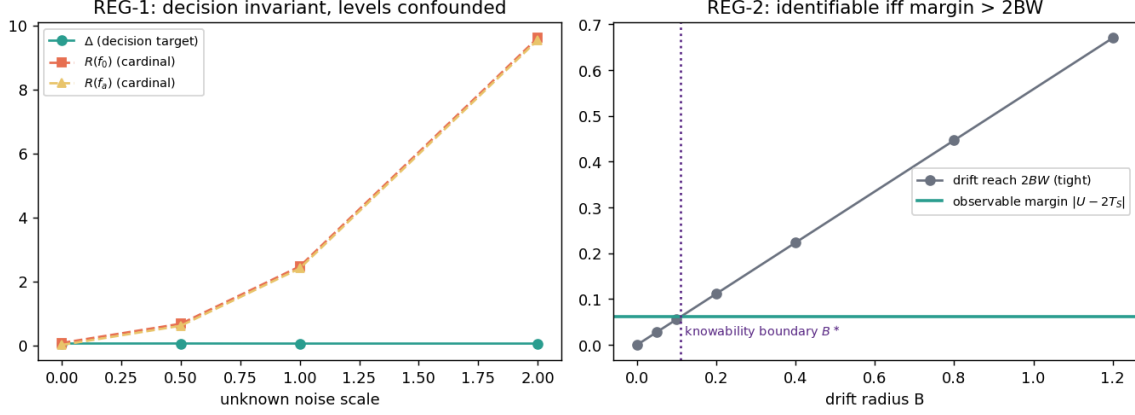
Figure 13: The bounded-drift knowability boundary (Theorem 17). Left: the decision target \Delta is invariant to unknown label noise while cardinal risks are confounded (Theorem 16). Right: identifiability holds exactly while the observable margin |U - 2T_S| exceeds the tight drift reach 2BW ; the crossing defines the computable boundary B^* .
