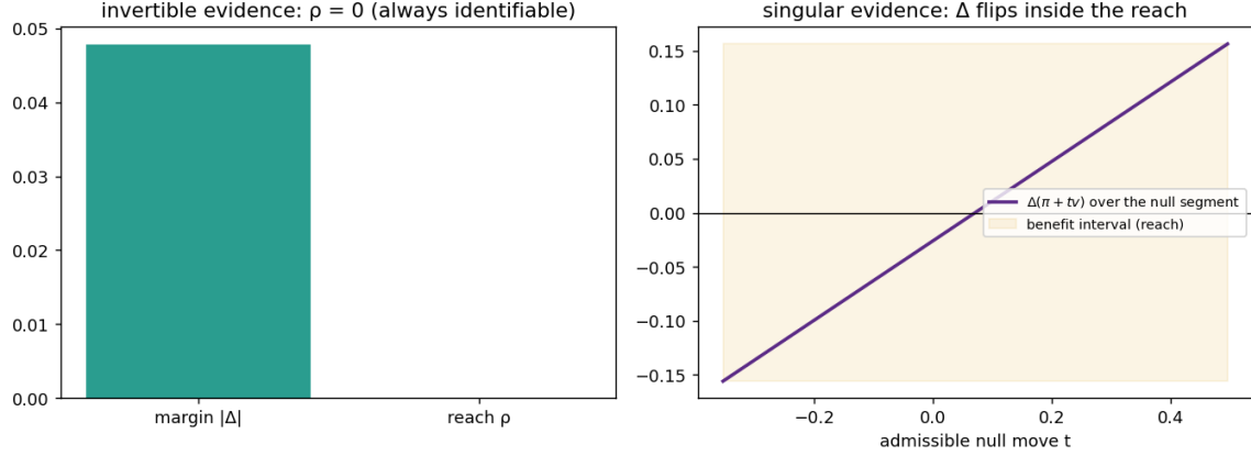
Figure 14: The label-shift boundary (Theorem 18). Left: injective evidence operator, reach 0 — always identifiable. Right: singular evidence; the benefit \Delta(\pi + tv) sweeps the reach interval along the unobservable null segment and crosses zero — identifiable exactly when the margin clears the reach.
