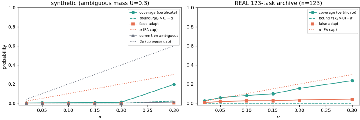
Figure 17: The knowability frontier (Theorem 21). Left: synthetic stream with planted ambiguous mass — false-adapt stays below \alpha , coverage dominates the \mathbb{P}[\kappa_\alpha > 0] - \alpha bound, and commits on ambiguous evidence respect the 2\alpha converse cap. Right: the same certificate on the real 123-task archive. Produced by scripts/knowability_frontier_validation.py .
