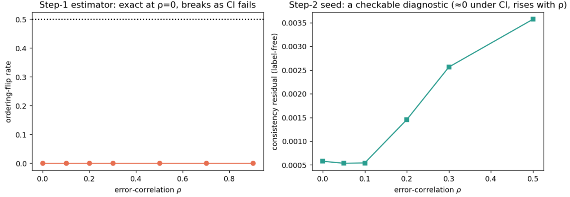
Figure 16: Multi-candidate identifiability (Theorem 20, Proposition 5). Left: the label-free ordering estimator is exact under conditional error-independence and degrades as it fails. Right: the overdetermination residual is a checkable diagnostic — \approx 0 under independence, rising with error-correlation.
