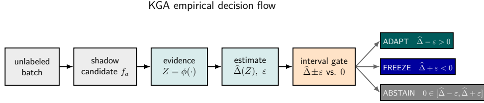
Figure 1: KGA’s empirical decision flow for one evaluation cell. A shadow adapter creates f_a from frozen f_0 . Labeled development cells fit the benefit predictor, and disjoint residual-calibration cells determine its error radius. The scored cell contributes label-free evidence only. An interval above zero selects ADAPT, one below zero selects FREEZE, and an interval crossing zero selects ABSTAIN. The figure defines the action rule; it does not establish interval coverage.
