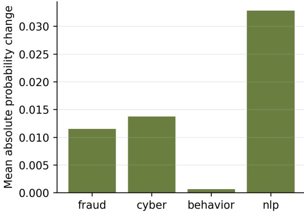
Fig. 13. Mean absolute counterfactual domain-attribution impact.
