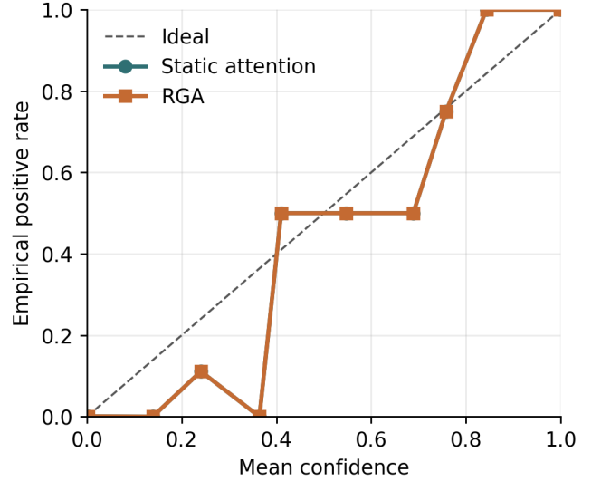
Fig. 14. Reliability diagram for static attention and RGA.
