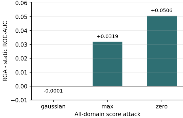
Fig. 11. All-domain adversarial ROC-AUC delta between RGA and static attention. Complete single-domain scenarios are reported in Table XXII.
