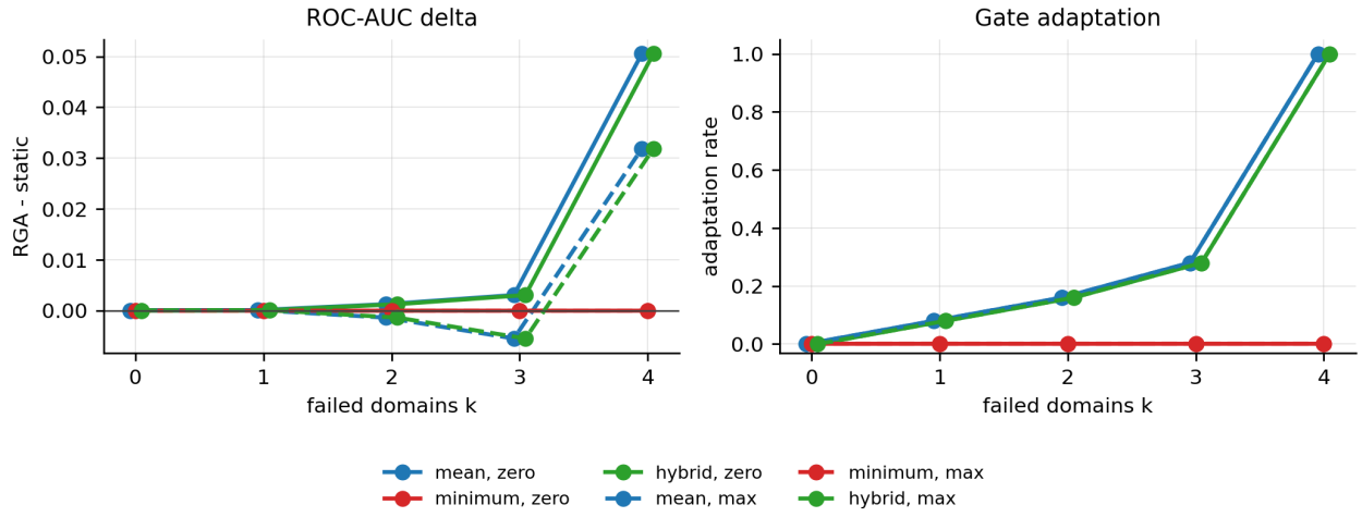
Fig. 12. k -of- D corruption mechanism evidence. The mean and hybrid gates show little reliable benefit for isolated or partial failures and activate fully only at all-domain collapse. The minimum gate remains closed at \tau_{\min} = 0.34 , exposing the current RGA-v2 threshold gap.
