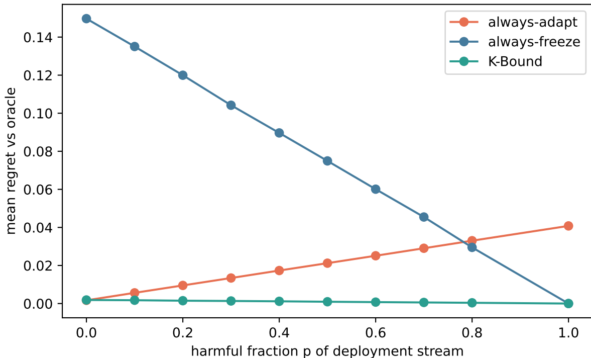
cifar10c (tent): Mixture-regret envelope across deployment mixes
