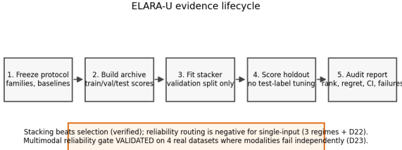
Fig. 10. Router decision lifecycle and evidence boundary. Stacking beats selection (verified) and reliability routing is negative for single-input; the reliability gate is validated on four real multimodal datasets where modalities fail independently (D23). Sealed external evidence still bounds any universal-SOTA claim.
