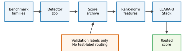
Fig. 8. ELARA-U architecture: benchmark families feed a detector zoo and score archive; validation-only labels and unlabeled deployment scores drive the router.
