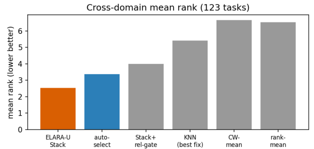
Fig. 1. Cross-domain mean rank over 123 tasks (lower better). ELARA-U Stack achieves the best average rank on the clean benchmark. (Illustrative; authoritative values in Table VI.)
