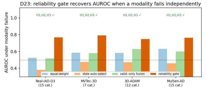
Fig. 7. Multimodal independent-modality-failure regime (D23) on four real datasets under the canonical noise protocol. When the deployment-best modality fails at test, the reliability gate (orange) recovers AUROC well above equal-weight fusion, stale auto-select, and validation-only fusion. “H1,H2,H3 ✓” marks datasets where all three pre-registered hypotheses pass — all four do. Authoritative deltas and CIs in Table XX.
