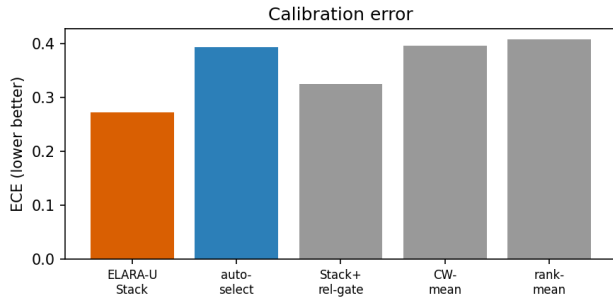
Fig. 3. Calibration error (ECE, lower better). ELARA-U Stack has the best raw ECE; fitted Brier/NLL in Table X.
