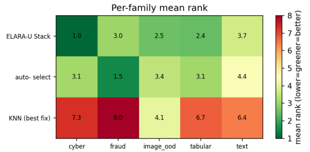
Fig. 5. Per-family mean rank (greener = better).
