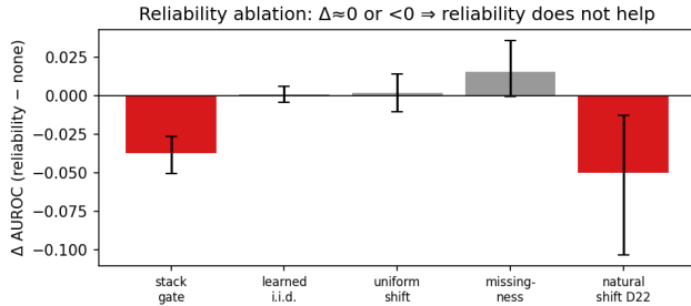
Fig. 6. Component ablation summary. The stack gain comes from rank-normalized per-task stacking; reliability/drift feature ablations are decisive and negative (Table XII). (Illustrative; authoritative values in Table XII.)
