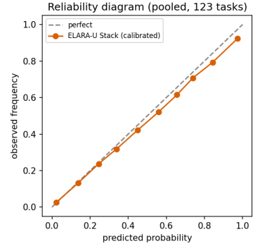
Fig. 4. Reliability diagram for the isotonic-calibrated ELARA-U Stack, pooled over 123 tasks (calibrator fit on validation only). Points near the diagonal indicate good calibration; Brier/NLL in Table X.
